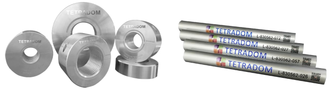
Quantum Ring
